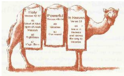
Camel Method
